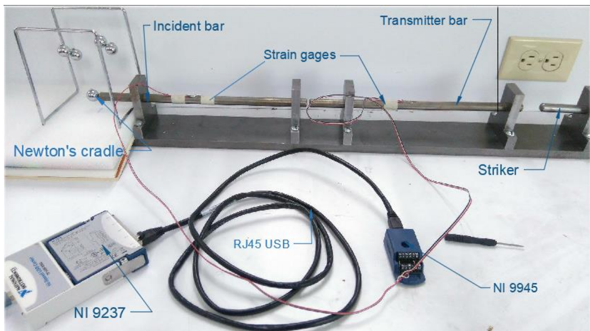
Figure 3. Equipment connected.
