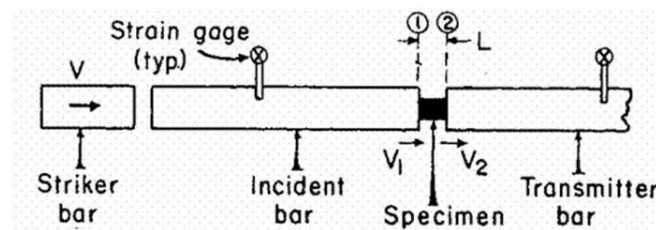
Figure 1. Schematic of a SHPB (Singh, 2009)
