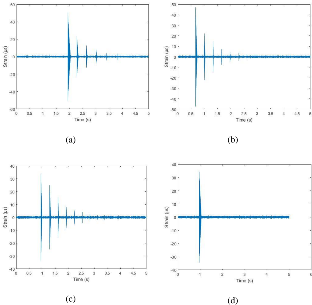
Figure 4. The graphs (a) and (b) shown the variation of strain through time in the incident and transmitter bar without contact; (c) and (d) shown the variation of strain with the bars in contact, (c) the incident bar and (d) the transmitter bar.
