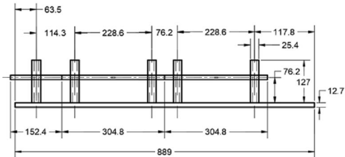
Figure 2. Designed SHPB in mm.
